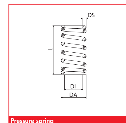
Pressure spring
